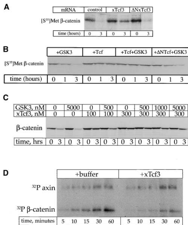
Figure 1. Tcf3 blocks \beta -catenin degradation in extracts and phosphorylation in vitro. (A) Translated Tcf3 but not \Delta NTcf3 mRNA inhibits \beta -catenin degradation in extracts. (B) Purified Tcf3 protein (1 \mu M) blocks \beta -catenin degradation. This effect was not reversed by 1 \mu M GSK3. Purified \Delta NTcf3 (1 \mu M) does not block \beta -catenin degradation. (C) Inhibition of \beta -catenin degradation by lower (100 nM) Tcf3 levels can be partially rescued by GSK3; higher Tcf3 (300 nM) levels cannot be rescued by even a large GSK3 excess. (D) Tcf3 inhibits the phosphorylation of \beta -catenin by GSK3 and axin in a purified system. In the same reaction, axin phosphorylation by GSK3 is not affected by Tcf3.
