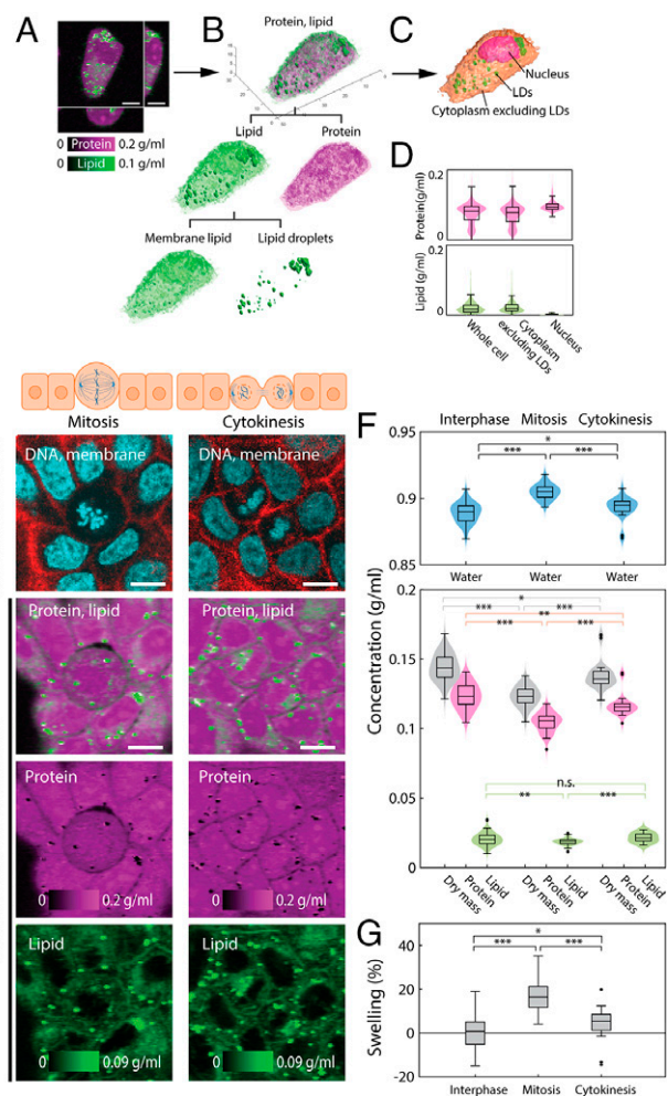
Fig. 2. Label-free measurement of protein and lipid shows dilution of cytoplasm in mitotic cells. (A) Volumetric NoRI measurement of a live A7 cell. (Scale bar, 10 \mu m.) (B) Volumetric visualization of the protein and lipid distribution in the cell. Lipid is further classified as membrane lipids in the aqueous phase of the cytosol and lipid droplets. (C) Label-free volumetric segmentation of a whole cell, nucleus, and lipid droplets from NoRI data. See SI Appendix, Supplementary Methods for the segmentation method. (D) Distribution of protein and lipid concentration within the volume of the whole cell, cytoplasm excluding lipid droplets, and the nucleus in C. (E) Representative live MDCK cells in mitosis and cytokinesis. (Scale bars, 10 \mu m.) (F) NoRI images of mitotic and interphase cells. Mitotic cells have a more diluted cytoplasm compared to interphase cells, as revealed by lower protein and lipid concentrations and a higher water concentration (water: interphase 0.889 \pm 0.008 g/mL, mitosis 0.905 \pm 0.006 g/mL, P < 0.0001 ; dry mass: interphase 0.144 \pm 0.009 g/mL, mitosis 0.123 \pm 0.007 g/mL, P < 0.0001 ; protein: interphase 0.123 \pm 0.009 g/mL, mitosis 0.105 \pm 0.007 g/mL, P < 0.0001 ; and lipid: interphase 0.021 \pm 0.005 g/mL, mitosis 0.019 \pm 0.002 g/mL, P = 0.0052 ). The cytoplasmic concentration recovers toward the interphase value during cytokinesis (water 0.893 \pm 0.008 g/mL, dry mass 0.138 \pm 0.010 g/mL, protein 0.117 \pm 0.008 g/mL, lipid 0.022 \pm 0.003 g/mL). Lipid droplets are excluded from the lipid concentration calculation. The number of cells in interphase, metaphase, and cytokinesis are n = 81 , n = 57 , and n = 24 , respectively. (G) Relative difference of cytoplasmic density, here expressed in terms of the relative volume change ("swelling") based on the degree that a cell of interphase cells' median cytoplasmic density would have to change to achieve the observed difference in cytoplasmic water concentration. Mean and SD of swelling are 0.5 \pm 6.8\% , 17.0 \pm 6.8\% , and 4.2 \pm 7.3\% for interphase, mitosis, and cytokinesis, respectively ( P < 0.001 for interphase and mitosis, P = 0.020 for interphase and cytokinesis). * P \leq 0.05 , ** P \leq 0.01 , *** P \leq 0.001 . n.s. is not significant with P > 0.05 .
